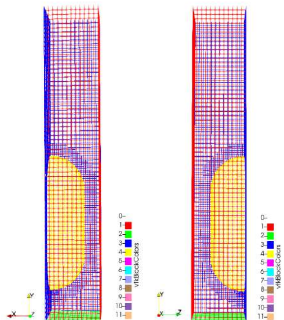
Fig. 1. (b) Back view (left) and side view (right) of symmetrical cut section of the elevator mesh (mesh view)
