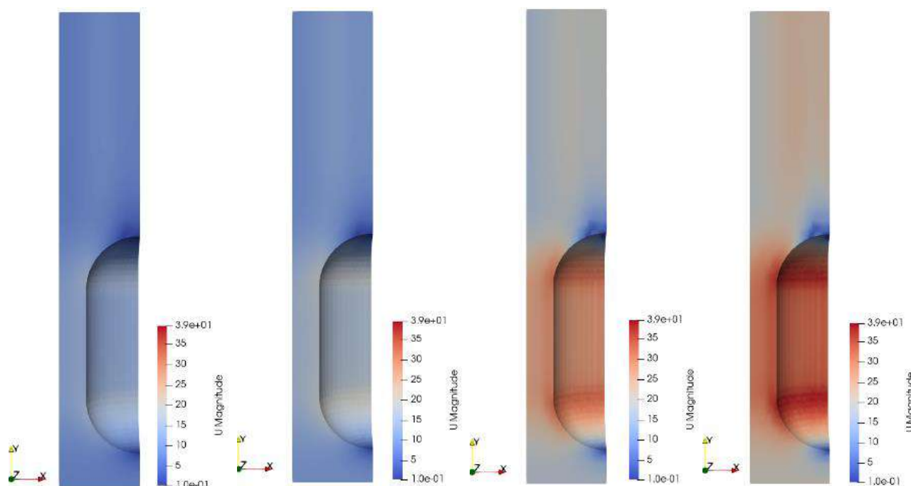
Fig. 2. (a) Velocity for rated speed of 8 m/s
