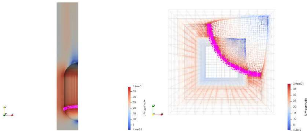
Fig. 5. The side view (left) and the bottom view (right) of the high air velocity and lower turbulence region highlighted in maroon for case rated car speed of 20 m/s
