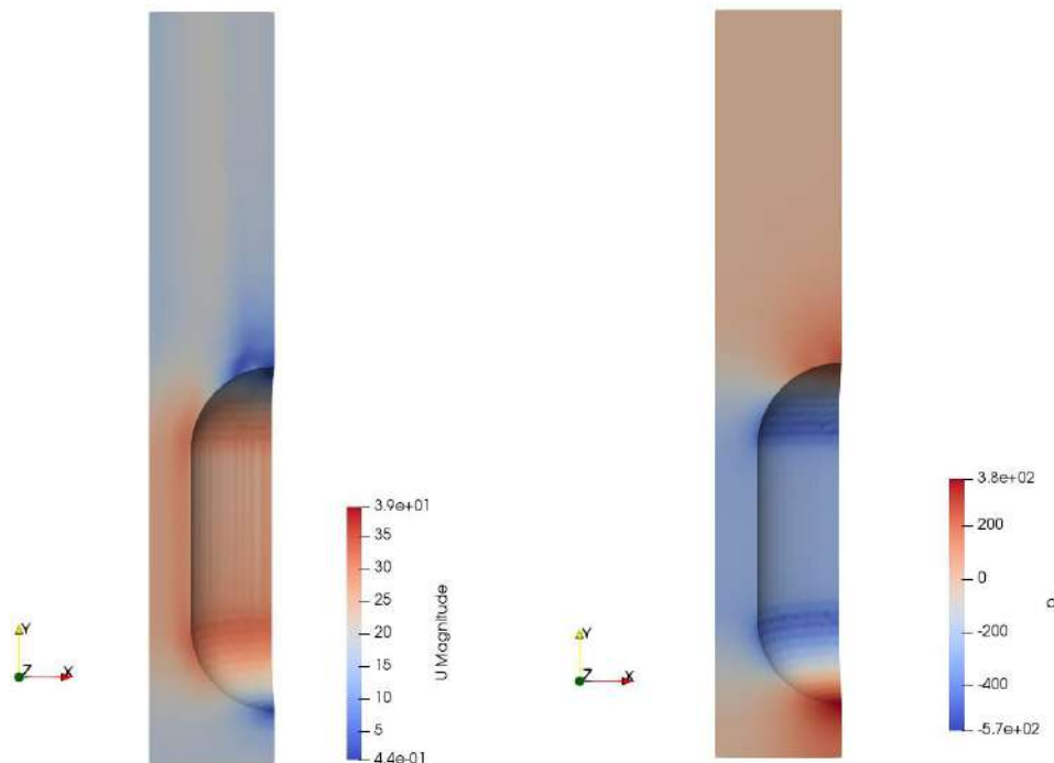
Fig. 7. Air velocity (left) and kinematic pressure (right) for car rated speed of 20 m/s
