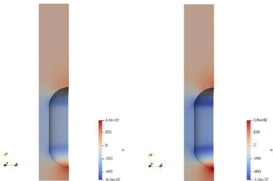
Fig. 6. Kinematic pressure for rated speed of 17 m/s (left) and 20 m/s (right)
