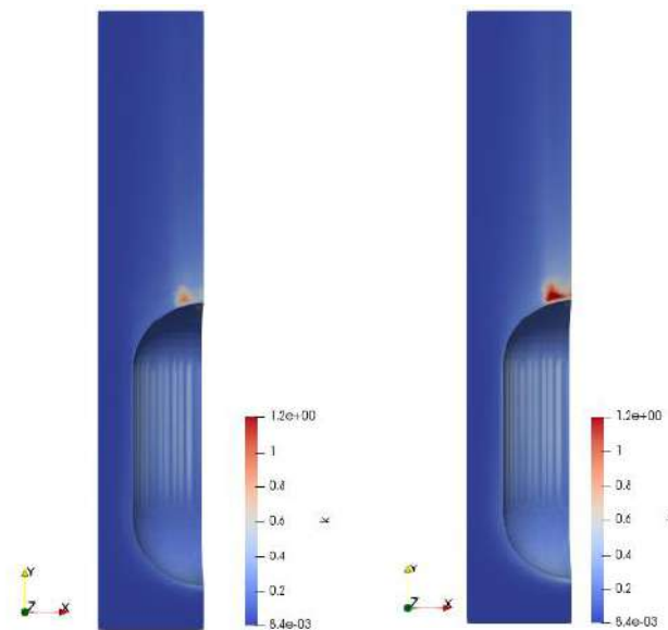
Fig. 3. Turbulence contour within the elevator system with the rated speed of 17 m/s (left) and 20 m/s (right)
