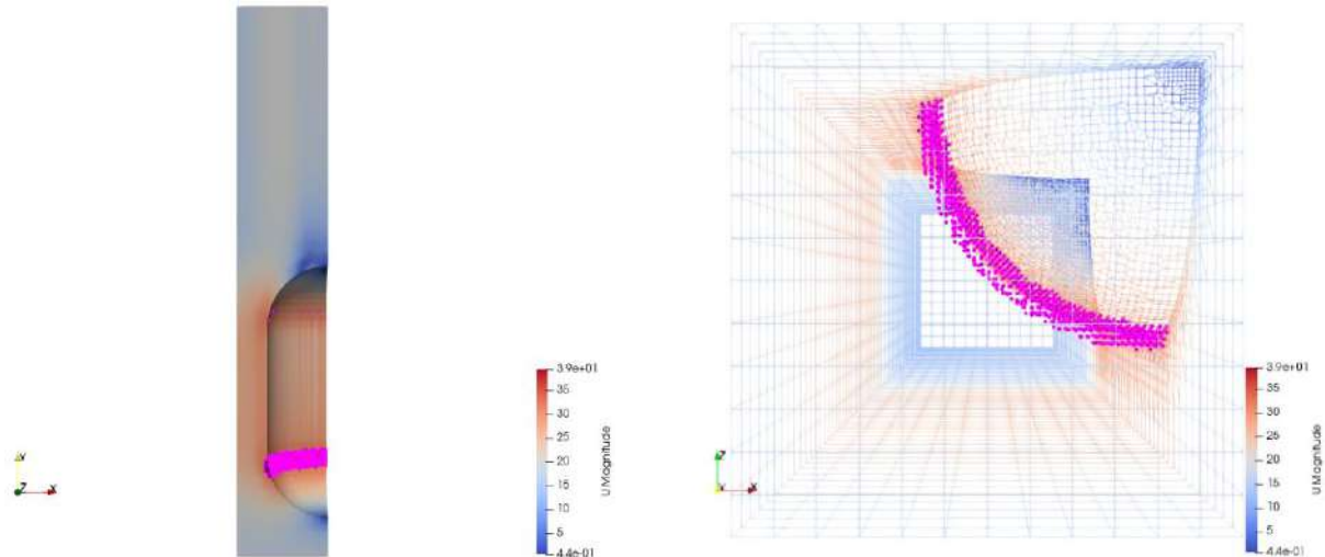
Fig. 4. The side view (left) and the bottom view (right) of the high air velocity and lower turbulence region highlighted in maroon for case rated car speed of 17 m/s
