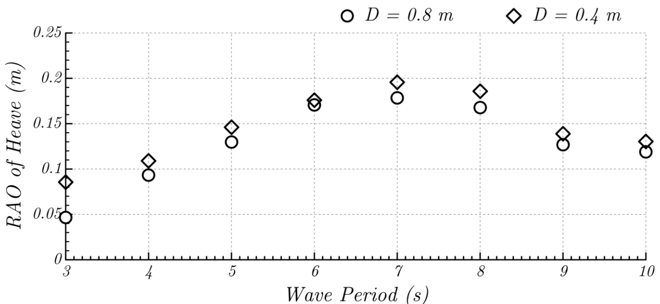
Fig. 7. Heave motion characteristics of floating jetty with and without heave plate at various drafts
