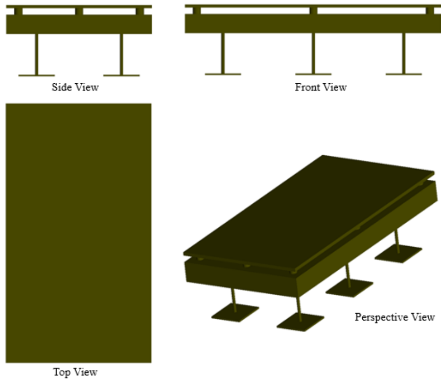
Fig. 1. Geometry of floating jetty incorporated with structural heave plate
