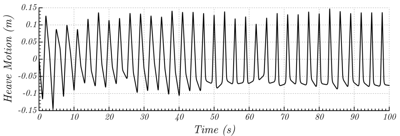
Fig. 3. Time history for heave motions of floating jetty at wave period of 4 seconds
