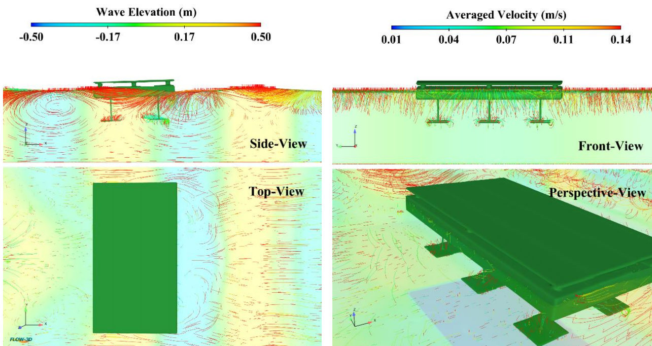
Fig. 4. Example CFD visualisation of floating jetty performances at wave periods of 4 seconds
