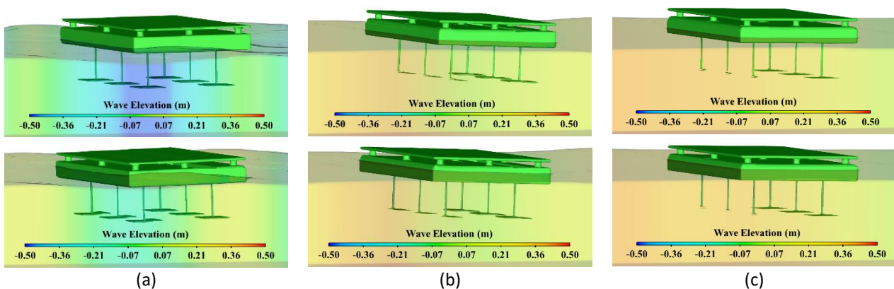
Fig. 8. Wave elevation characteristics of floating jetty incorporated with heave plate in different drafts; 0.4 m (above) and 0.8 m (below) at various wave periods for (a) T_w = 3s , (b) T_w = 6s and (c) T_w = 9s
