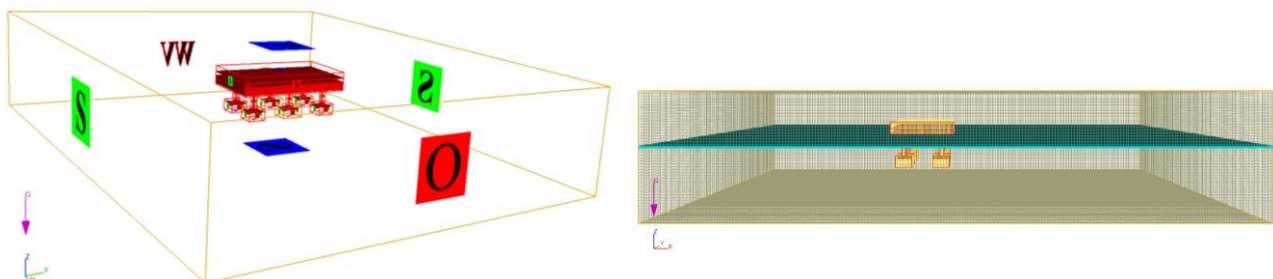
Fig. 2. Boundary condition (left) and mesh generation (right)
