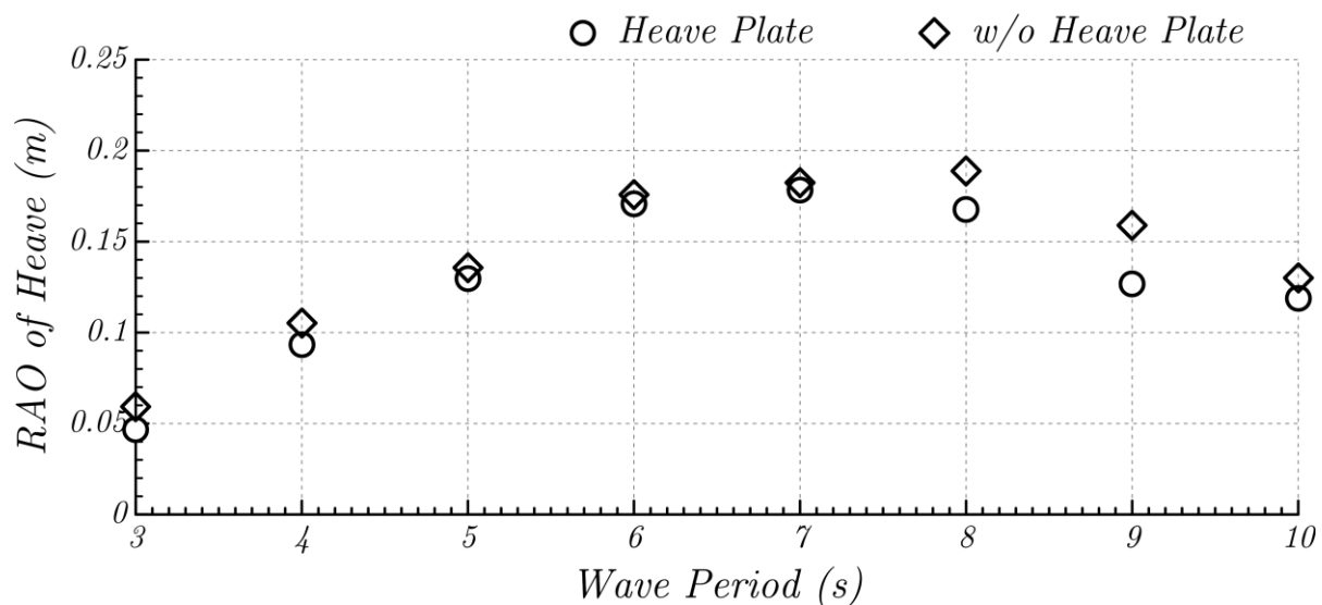
Fig. 5. Heave motion characteristics with and without heave plate at various wave periods
