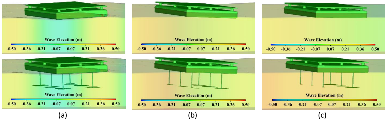
Fig. 6. Wave elevation characteristics of floating jetty without (above) and with (below) heave plates at various wave periods for (a) T_w = 3s , (b) T_w = 6s and (c) T_w = 9s
