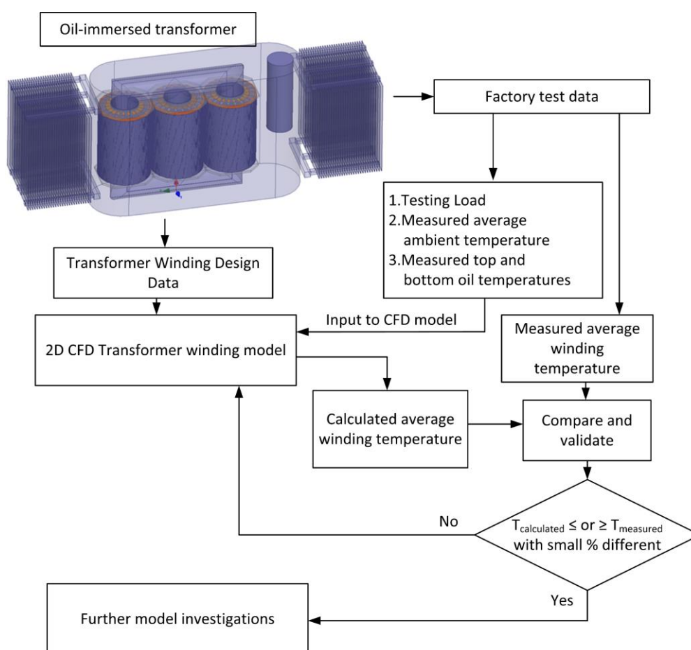
Fig. 1. Methodology chart
