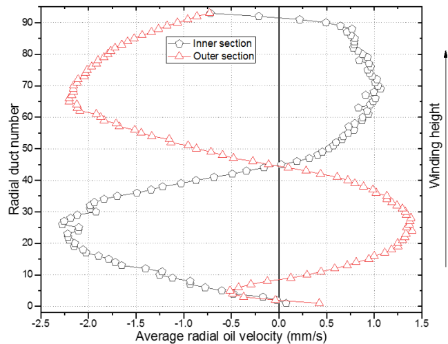
Fig. 10. Average radial oil flow velocity
