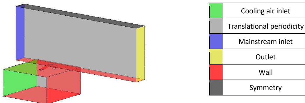
Fig. 3. Boundary conditions
