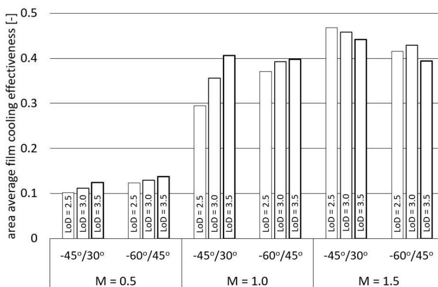
Fig. 11. Area average film cooling effectiveness
