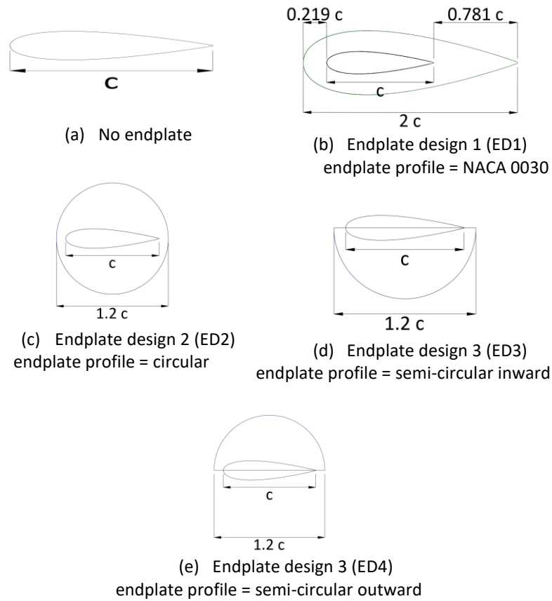
Fig. 3. Various blade tip designs
