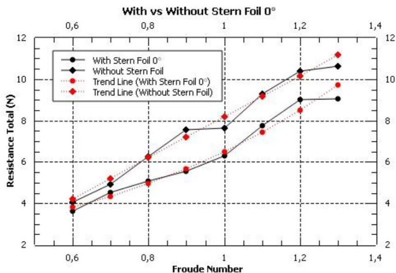
Fig. 9. Comparison application of stern foil using 0 ° angle
