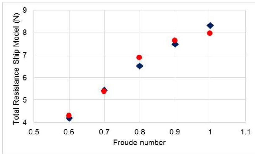
Fig. 5. Validation of simulation results with the previous experimental results
