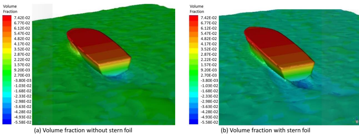
Fig. 8. Volume of Fraction comparison without and using stern foil 3° (stern view)
