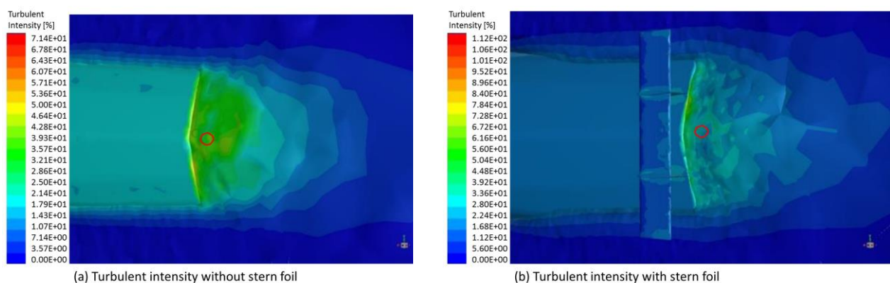
Fig. 6. Turbulent intensity stern foil 0° with 2 kg loading condition on Froude Number 0.9
