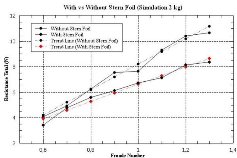
Fig. 10. Comparison application of stern foil using 3 ° angles
