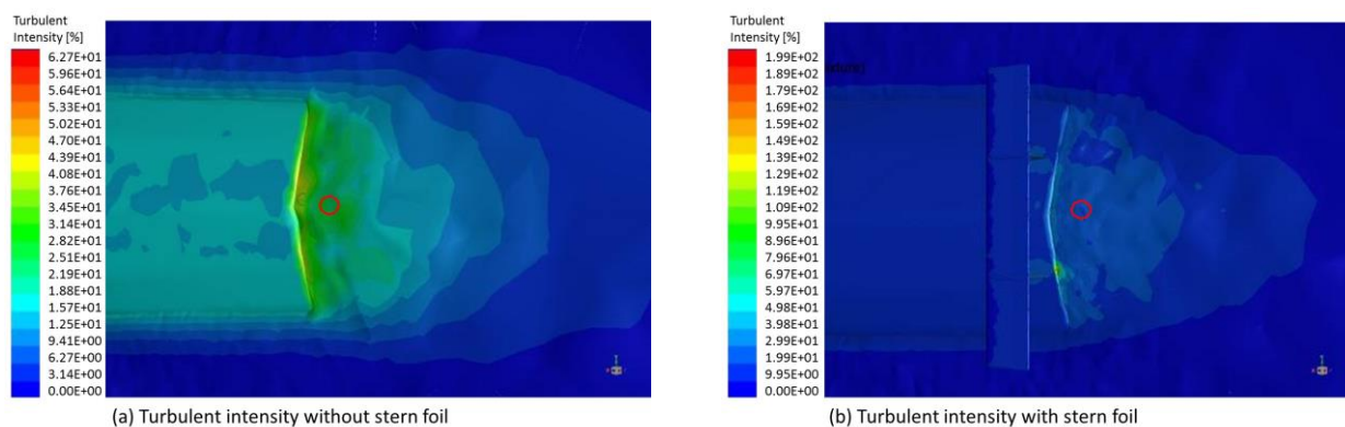
Fig. 7. Turbulent intensity stern foil 3° with 2 kg loading on Froude Number 1.1
