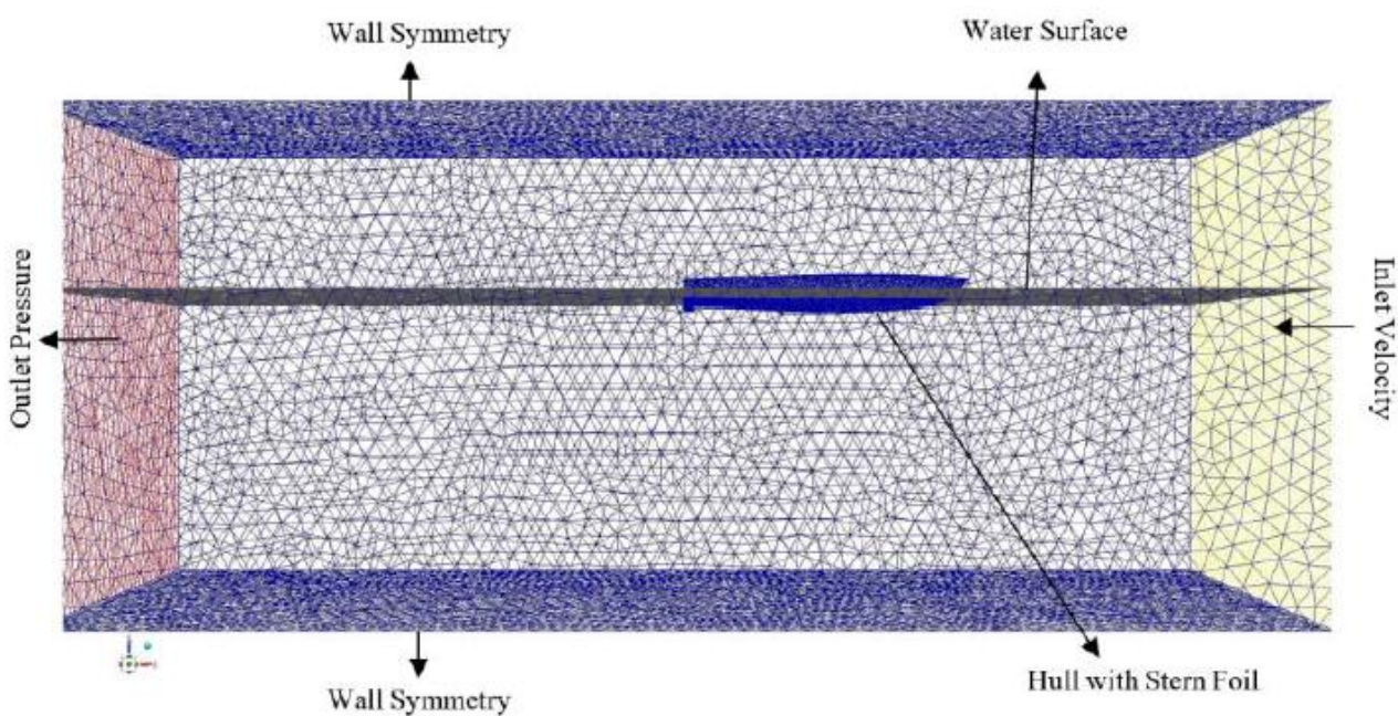
Fig. 4. Boundary condition of simulation model
