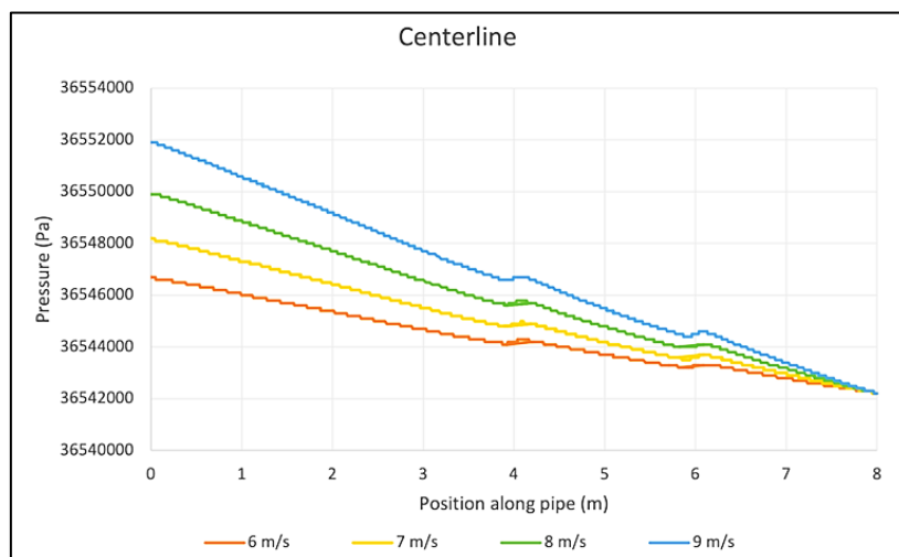
Fig. 23. Pressure behavior around the leaks between different fluid velocity along the pipe at centerline below the leaks
