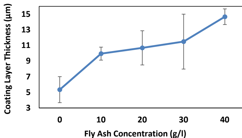
Fig. 3. Effect of fly ash concentration on the coating layer thickness
