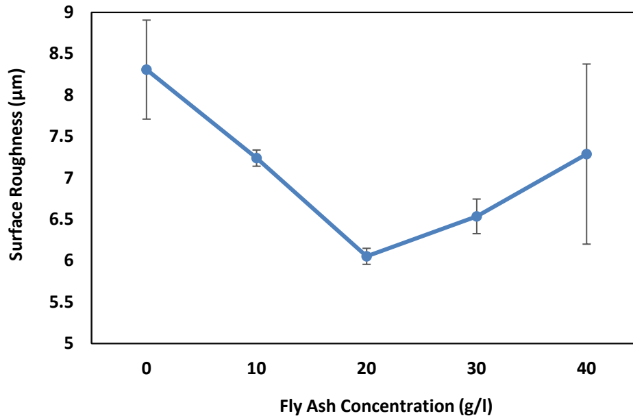
Fig. 5. Effect of fly ash concentration on the surface roughness
