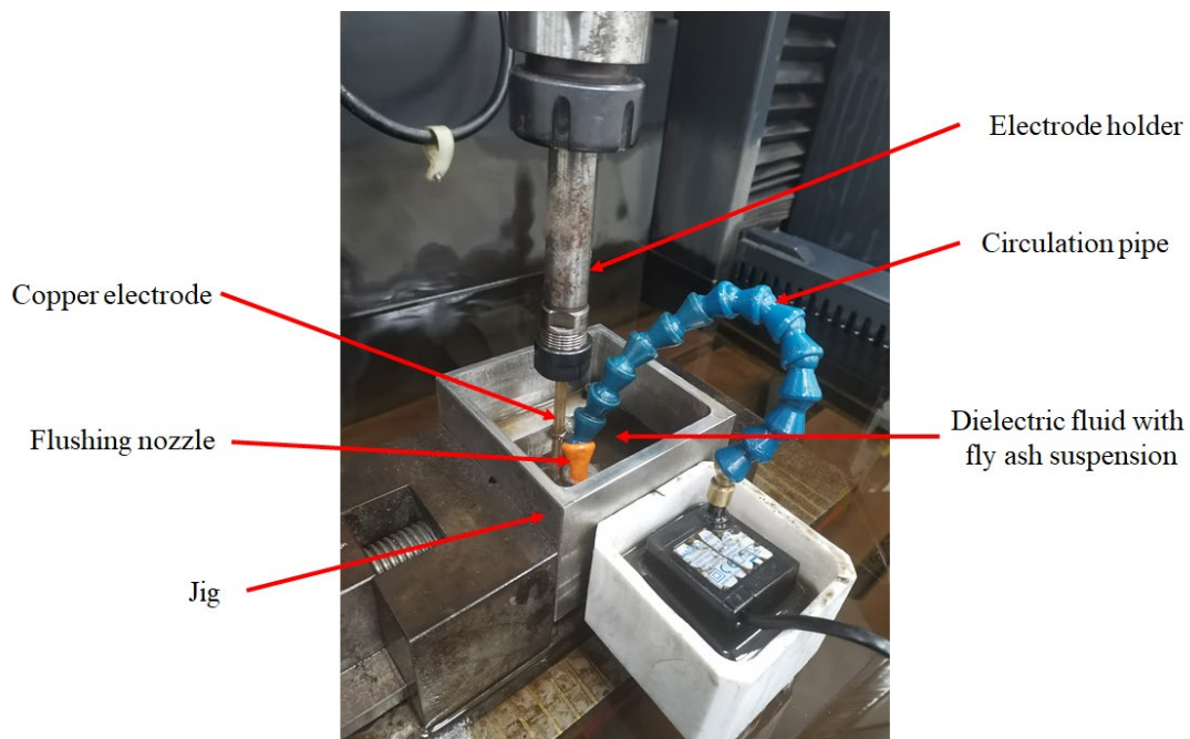
Fig. 2. Experimental setup
