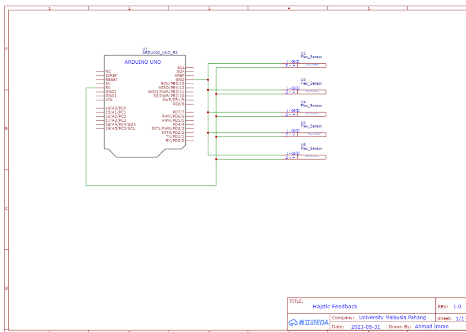
Fig. 2. Schematic circuit diagram
