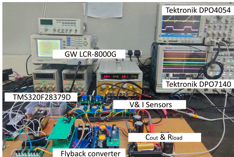
Fig. 8. Experiment setup
