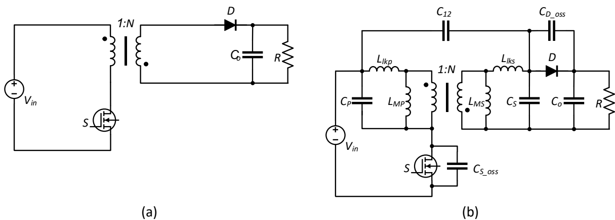
Fig. 3. (a) Basic flyback converter circuit typically used in PV microinverter and (b) common flyback converter with parasitic elements
