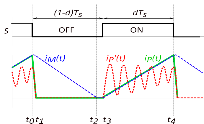
Fig. 4. Typical current response of a flyback converter
