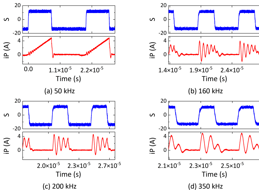
Fig. 9. Converter's primary current i_p with diverse switching frequencies: (a) 50 kHz, (b) 160 kHz, (c) 200 kHz, and (d) 350 kHz
