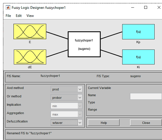
Fig. 8. FLC-PI design
