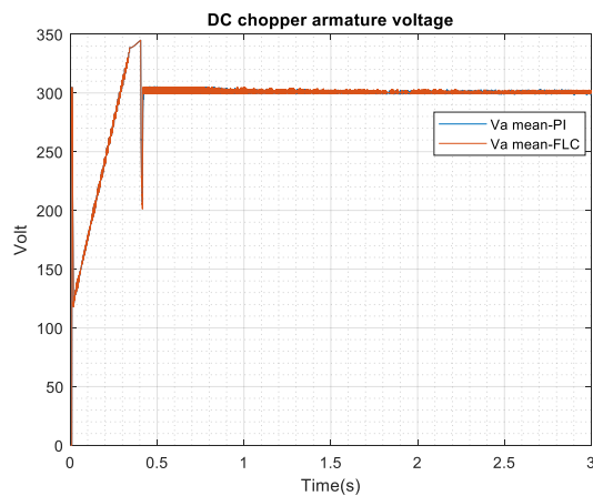
Fig. 22. Armature voltage performance with load of 100 Nm
