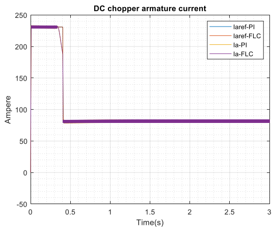
Fig. 20. Armature Current performance with load of 100 Nm
