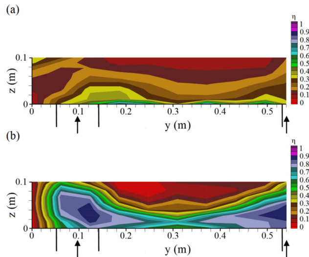
Figure 6: Film-cooling effectiveness distribution of plane 1p for (a) baseline case and (b) Case 2
