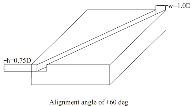
Figure 2: Schematic geometry of row trenched cooling holes with alignment angle of +60 degrees
