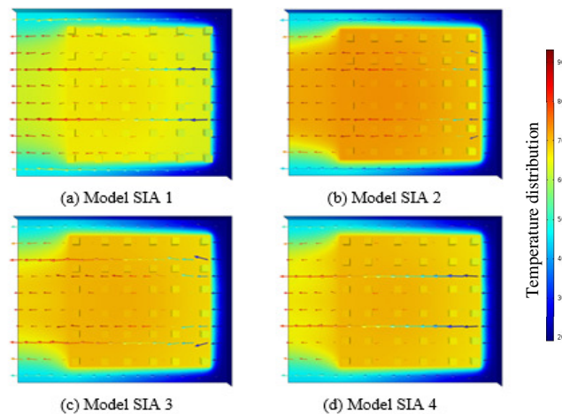
Figure 12: Top view plot of temperature and airflow for SIA of pin fin heat sink models. (a) Model SIA 1 (max temp: 90.211^{\circ}\text{C} ); (b) Model SIA 2 (max temp: 98.637^{\circ}\text{C} ); (c) Model SIA 3 (max temp: 95.385^{\circ}\text{C} ); (d) Model SIA 4 (max temp: 95.152^{\circ}\text{C} )
