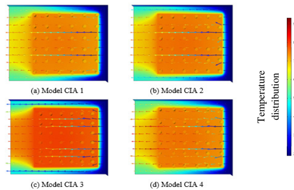
Figure 9: Top view plot of temperature and airflow for CIA of pin fin heat sink models. (a) Model CIA 1 (max temp: 101.03^{\circ}\text{C} ); (b) Model CIA 2 (max temp: 102.41^{\circ}\text{C} ); (c) Model CIA 3(max temp: 107.43^{\circ}\text{C} ); (d) Model CIA 4(max temp: 102^{\circ}\text{C} )
