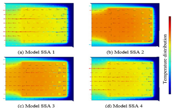
Figure 13: Top view plot of temperature and airflow for SSA of pin fin heat sink models. (a) Model SSA 1 (max temp: 90.399^{\circ}\text{C} ); (b) Model SSA 2 (max temp: 101.2^{\circ}\text{C} ); (c) Model SSA 3 (max temp: 98.702^{\circ}\text{C} ); (d) Model SSA 4 (max temp: 91.023^{\circ}\text{C} )
