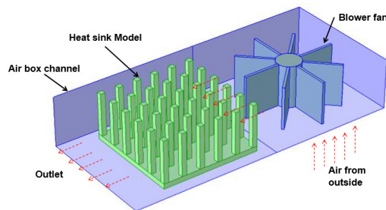
Figure 1: Simulation design set up
