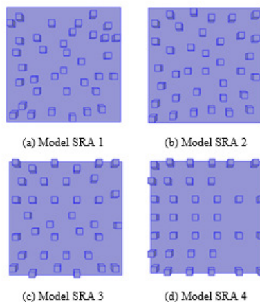
Figure 8: Top view of SRA pin fin models
