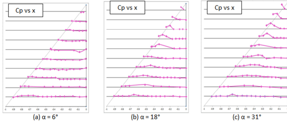
Fig. 7. Pressure distribution for large leading edge at Re = 1 \times 10^6
