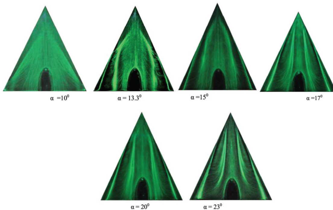
Fig. 2. Flow topology above large-edged wing at Reynolds number of 1 \times 10^6 , \alpha varies from 10^\circ to 23^\circ [3,13]
