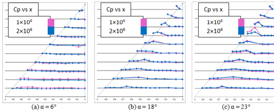
Fig. 10. Pressure distribution for large leading edge
