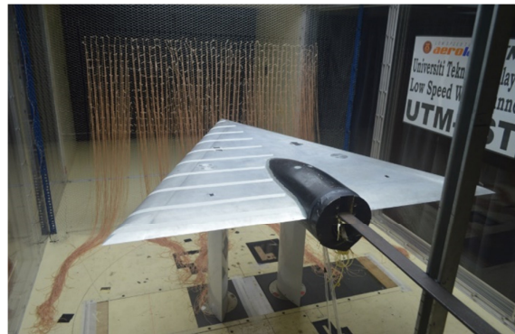
Fig. 6. Complete setup of tuft method
