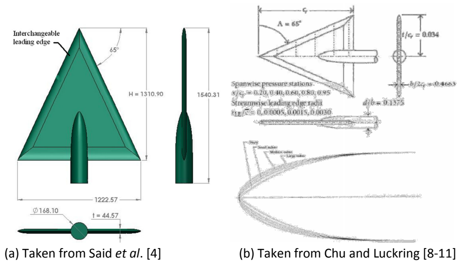
Fig. 3. (a) UTM-LST delta wing VFE-2 profiles (b) Original Chu and Lucking profile [8-11]
