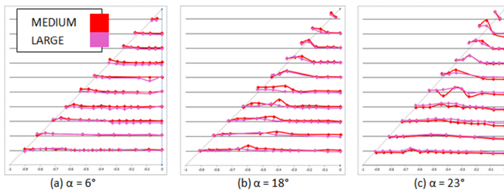
Fig. 11. Pressure distribution at Re = 1 \times 10^6 .
