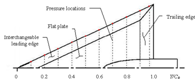
Chord-wise surface pressure locations: Y/C_R = 0.1, 0.2, 0.3, 0.4, 0.5, 0.6, 0.7, 0.8, 0.97
