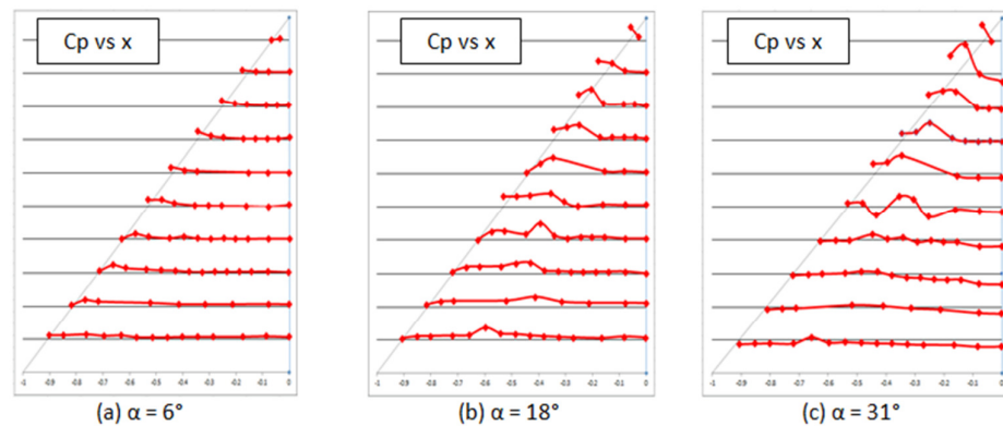
Fig. 9. Pressure distribution for medium leading edge at Re = 1 \times 10^6
