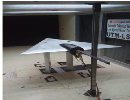
Fig. 4. Installation of UTM VFE-2 model at \alpha=5^\circ
