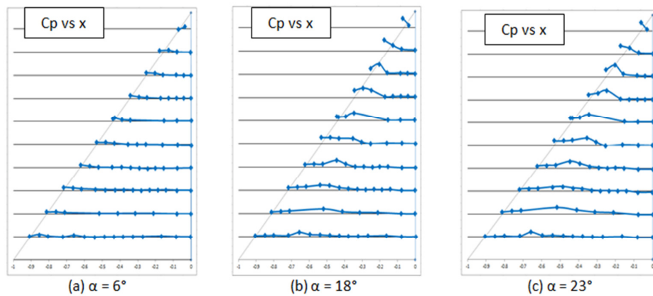
Fig. 8. Pressure distribution for large leading edge at Re = 2 \times 10^6
