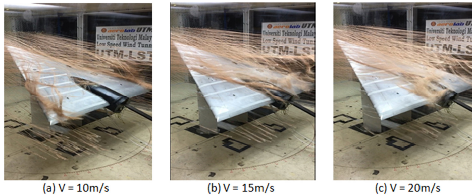
Fig. 12. Flow visualization at \alpha = 23^\circ
