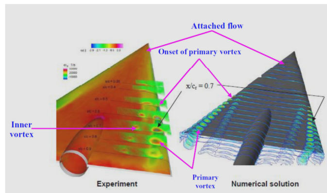
Fig. 1. Comparison of experimental measurement and Numerical studies above VFE-2 configurations at \alpha=13^\circ [2]
