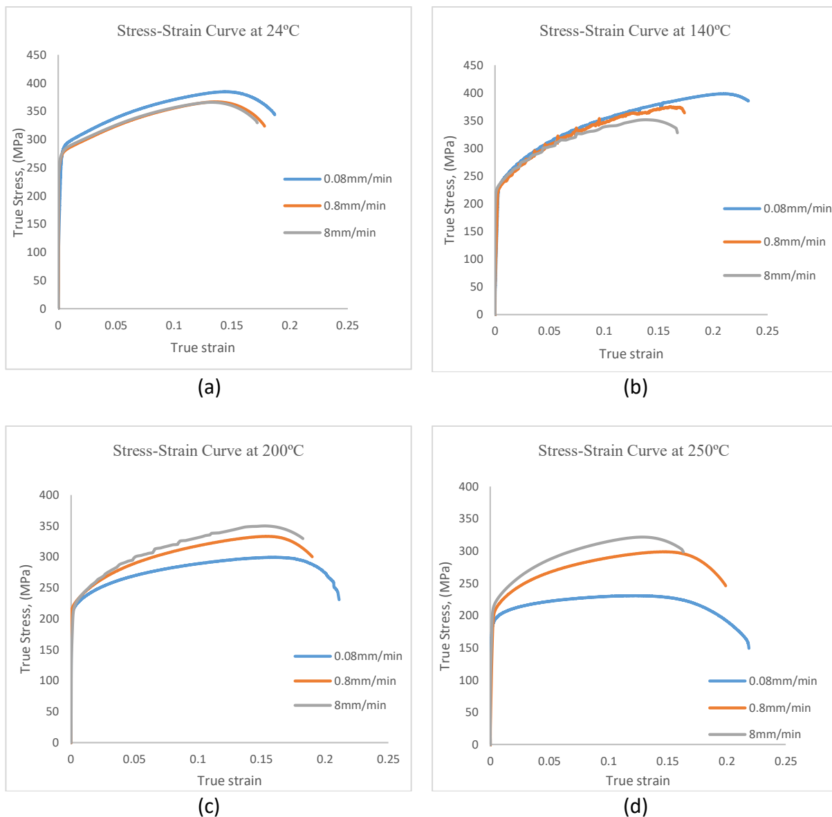
Fig. 4. (a-d) AA6061 Stress-Strain curves at different strain rates and temperature
