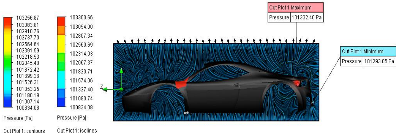
Fig. 5. Pressure contours and isolines across the photogrammetric car model
