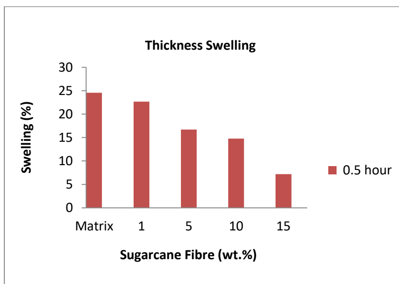
Fig. 3. Thickness Swelling for TPPS/sugarcane fibre composites
