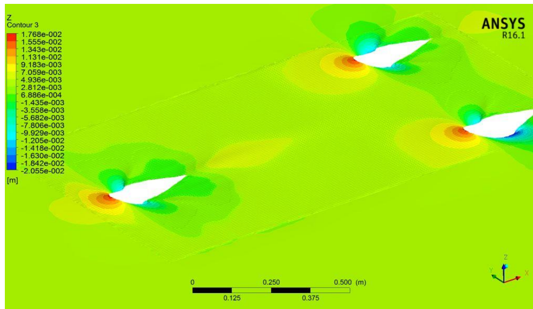
Fig. 14. Free surface at hull speed, V = 0.6\text{ms}^{-1}
