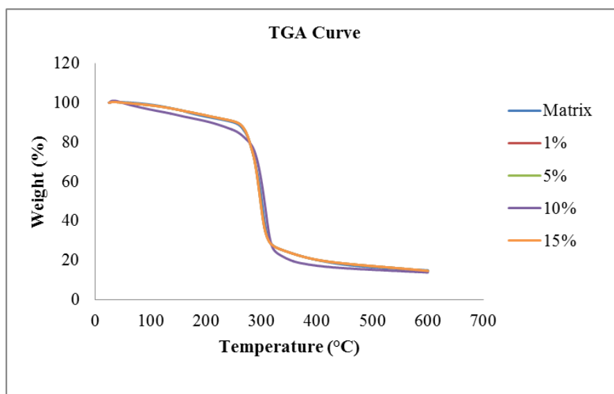
Fig. 1. TGA Curve for TPPS and TPPS/Sugarcane Fibre Composites
