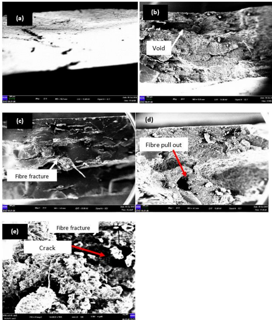
Fig. 8. SEM investigation of tensile fracture surface of TPPS/sugarcane fibre composites (a) TPPS matrix (b) 1 wt.% sugarcane fibre (c) 5 wt.% sugarcane fibre (d) 10 wt.% sugarcane fibre (e) 15 wt.% sugarcane fibre
