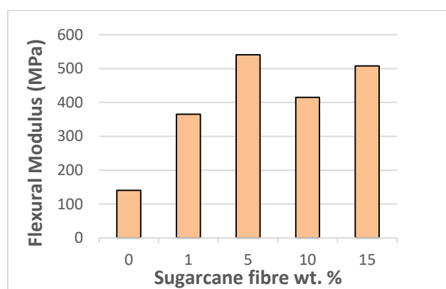
Fig. 7. Flexural modulus of TPPS/sugarcane fibre composites
