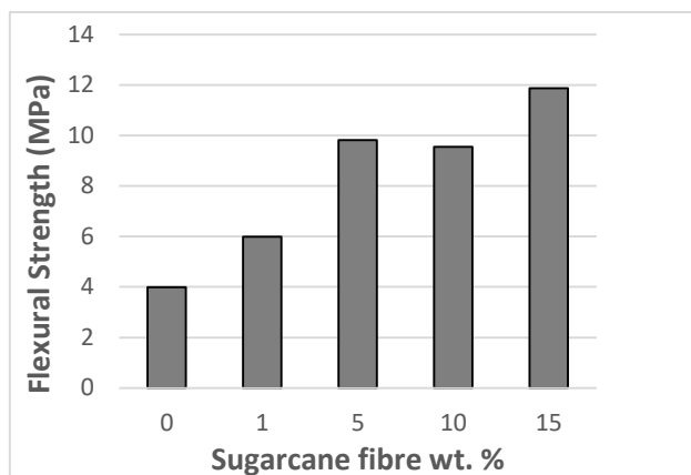
Fig. 6. Flexural strength of TPPS/sugarcane fibre composites
