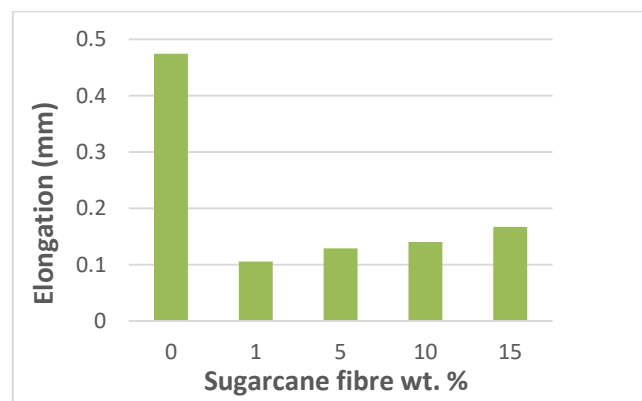
Fig. 5. Elongation at break of TPPS/sugarcane fibre composites
