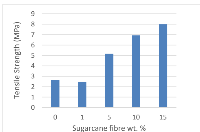
Fig. 3. Tensile strength of TPPS/sugarcane fibre composites
