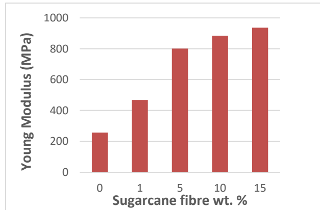
Fig. 4. Tensile modulus of TPPS/sugarcane fibre composites
