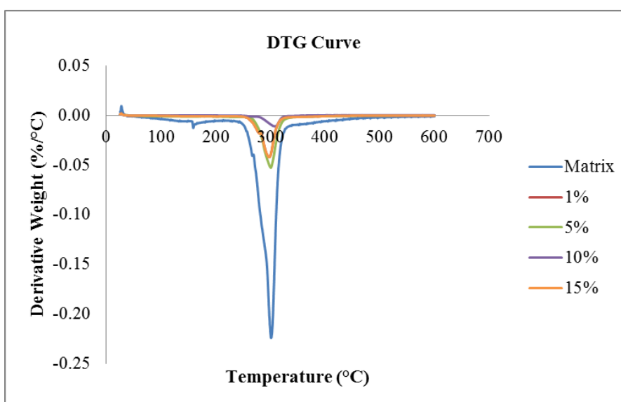
Fig. 2. DTG Curve for TPPS and TPPS/SF Composites
