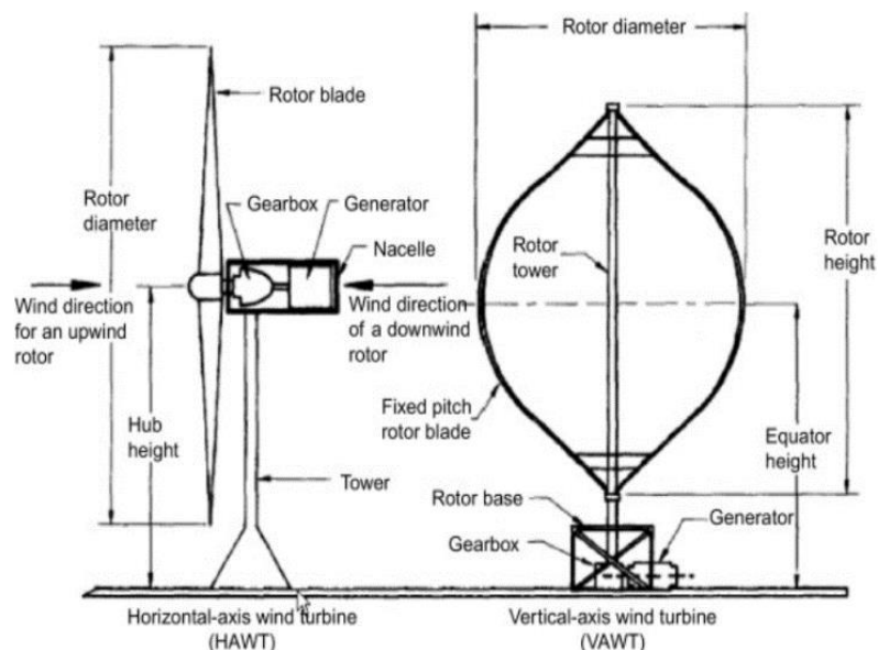
Fig. 1. Basic of HAWT and VAWT configurations [14]
