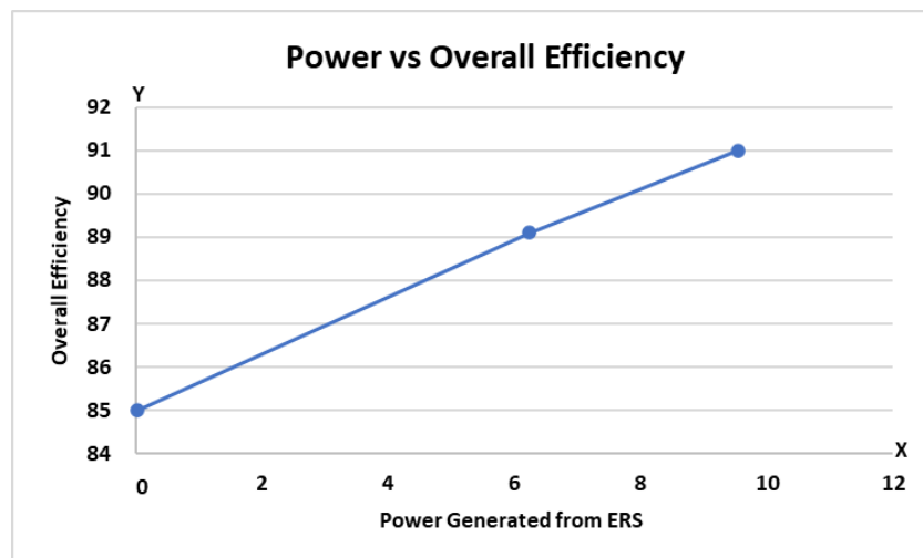
Fig. 9. Power vs Overall Efficiency [64]
