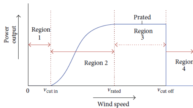
Fig. 5. Typical Wind Turbine Power Curve [25]
