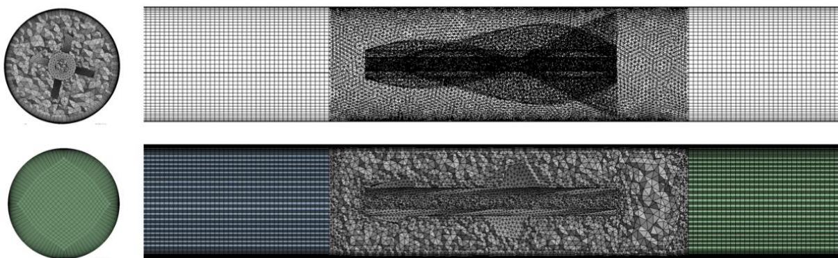
Fig. 6. Mesh Generation
