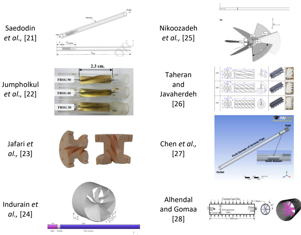
Fig. 3. Decaying swirlers
