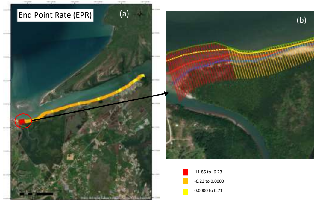
Fig. 6. End Point Rate analysis. a) EPR result along the study site, b) EPR for high erosion area
