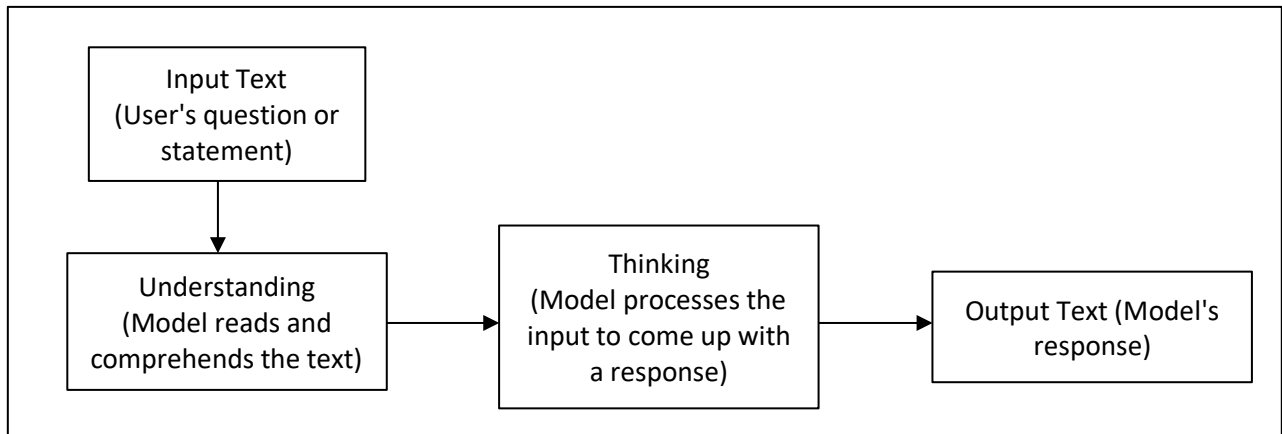
Fig 1. ChatGPT architectures
