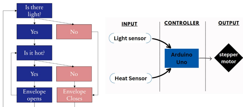
Fig. 7. The circuit logic diagram of how the DFED system operates with the input-to-output sequences and type of sensor used
