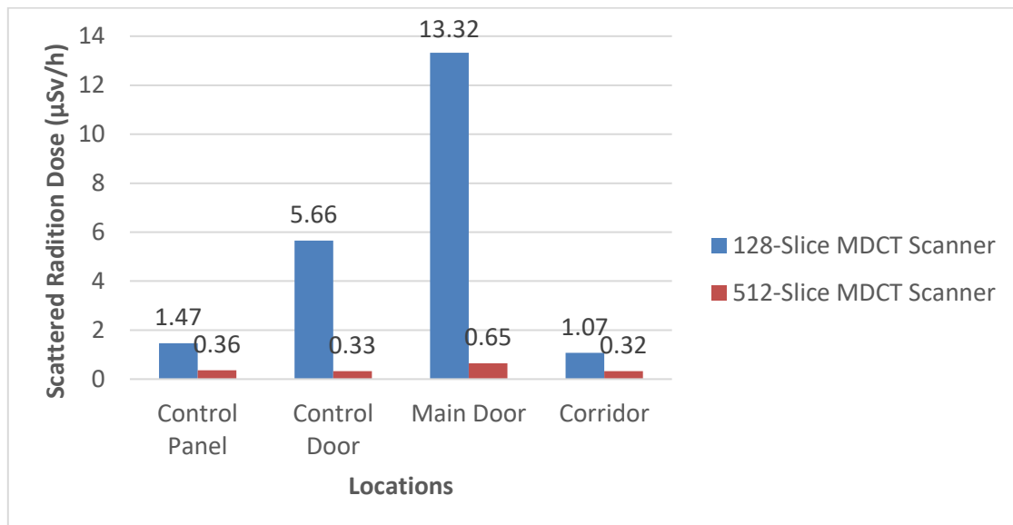
Fig. 1. Scattered radiation dose levels for CT brain imaging protocols at various locations in CT suite
