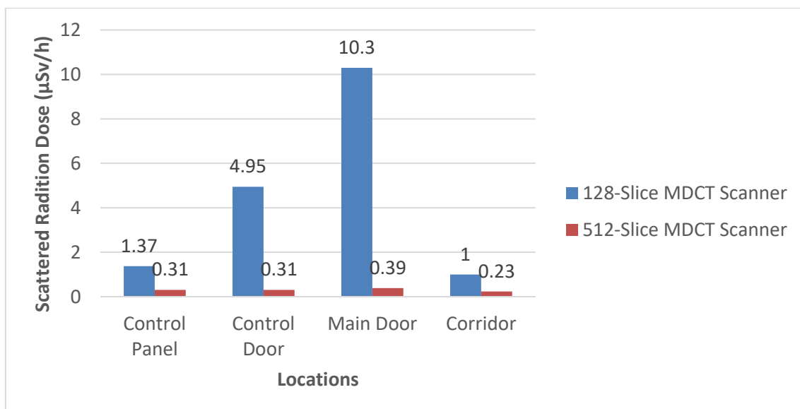
Fig. 3. Scattered radiation dose levels for CT abdomen imaging protocols at various locations in CT suite
