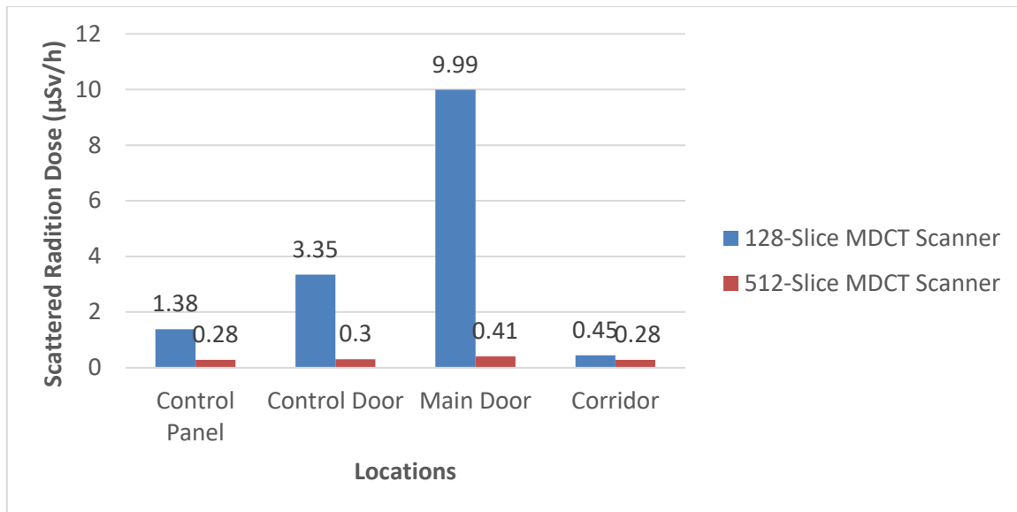
Fig. 2. Scattered radiation dose levels for CT thorax imaging protocols at various locations in CT suite
