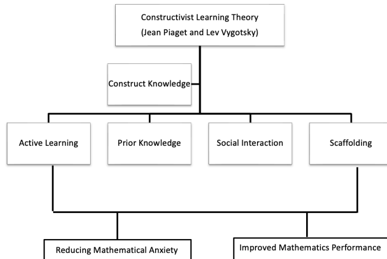
Fig. 1. Theoretical framework
