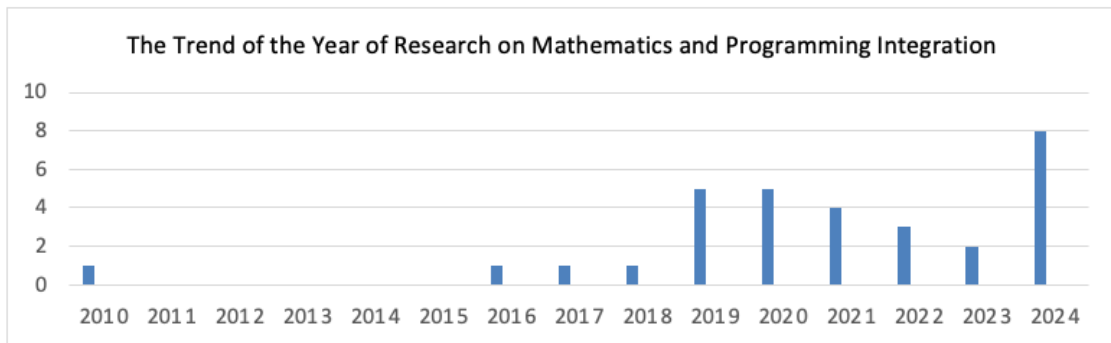
Fig. 4. The trend of the year of research on mathematics and programming integration
