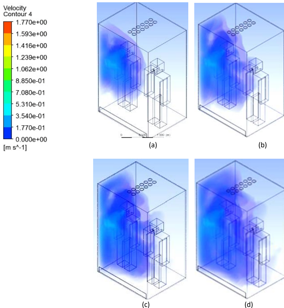
Fig. 5. The velocity distribution of the Corona Virus dispersion for (a) Case 1, velocity 1m/s (b) Case 2, velocity 2m/s (c) Case 3, velocity 3m/s (d) Case 4, velocity 4.5m/s
